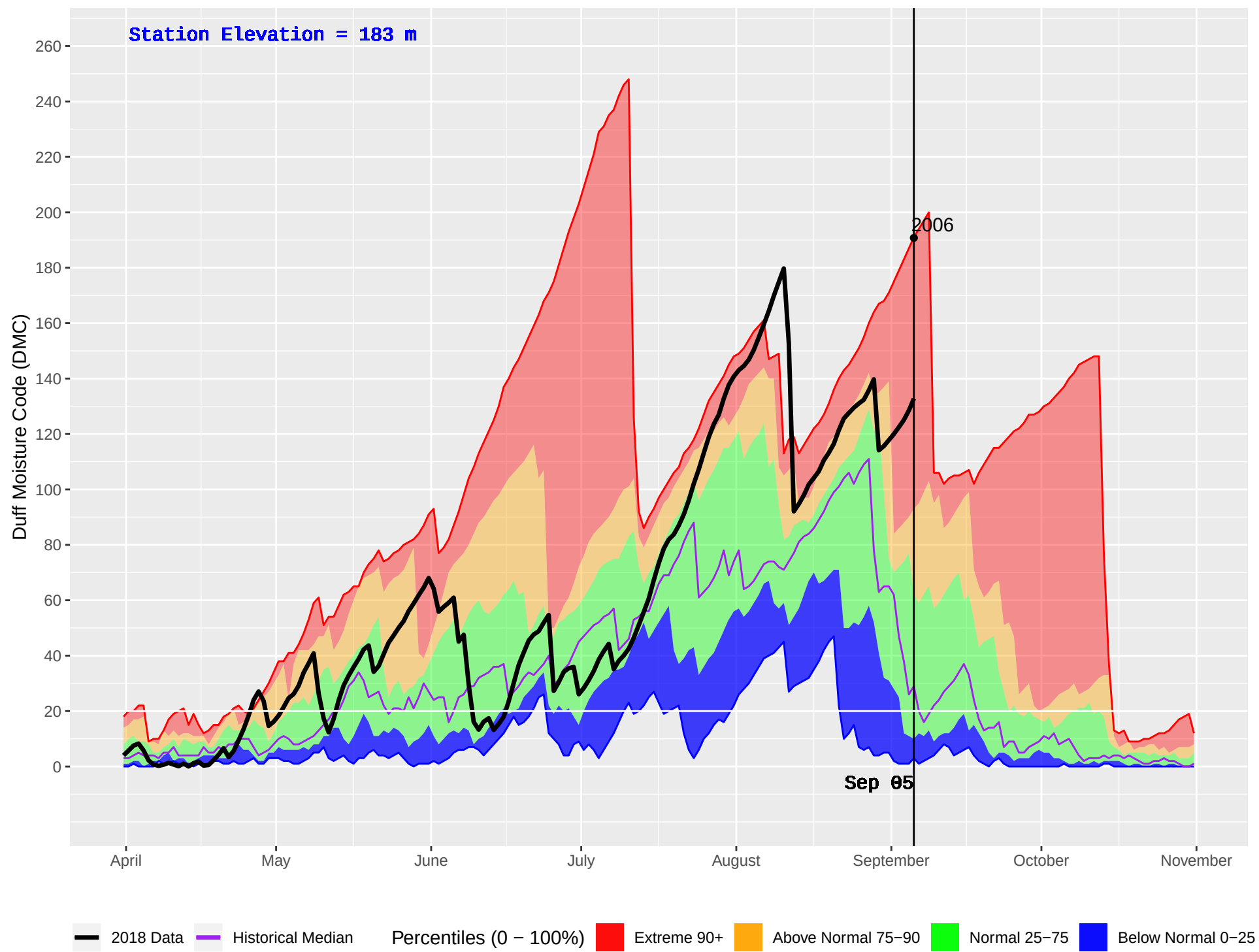
MESACHIE 2 (934) : Historical (2006–2016) and Current (2018) Daily Duff Moisture Code (DMC)
