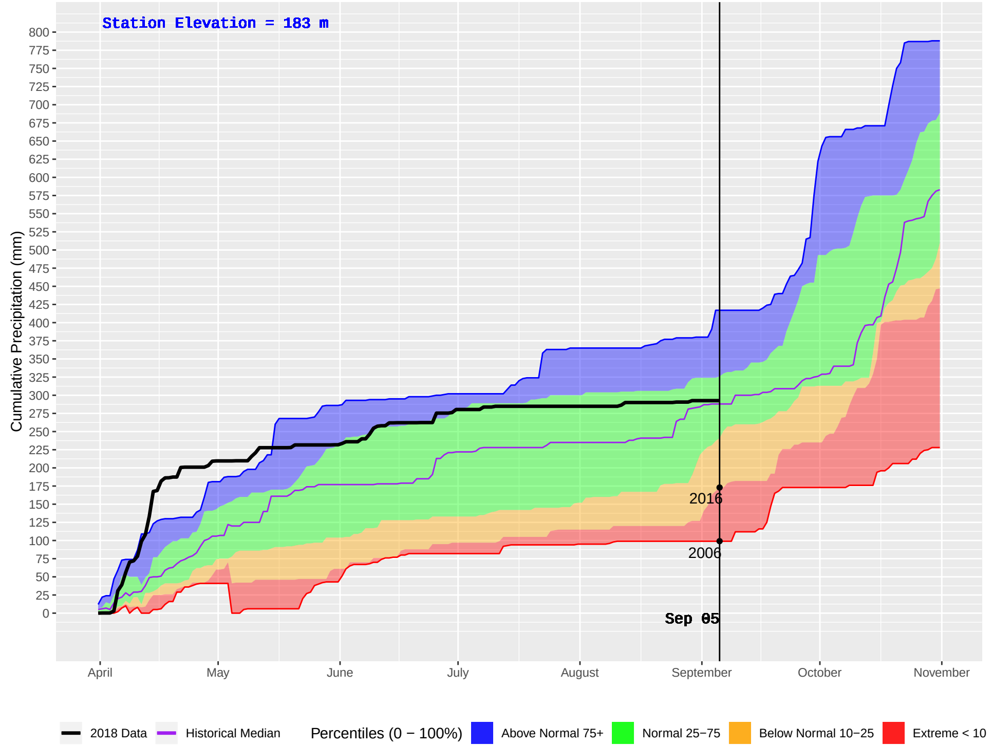
MESACHIE 2 (934) : Historical (2006–2016) and Current (2018) Daily Cumulative Precipitation
