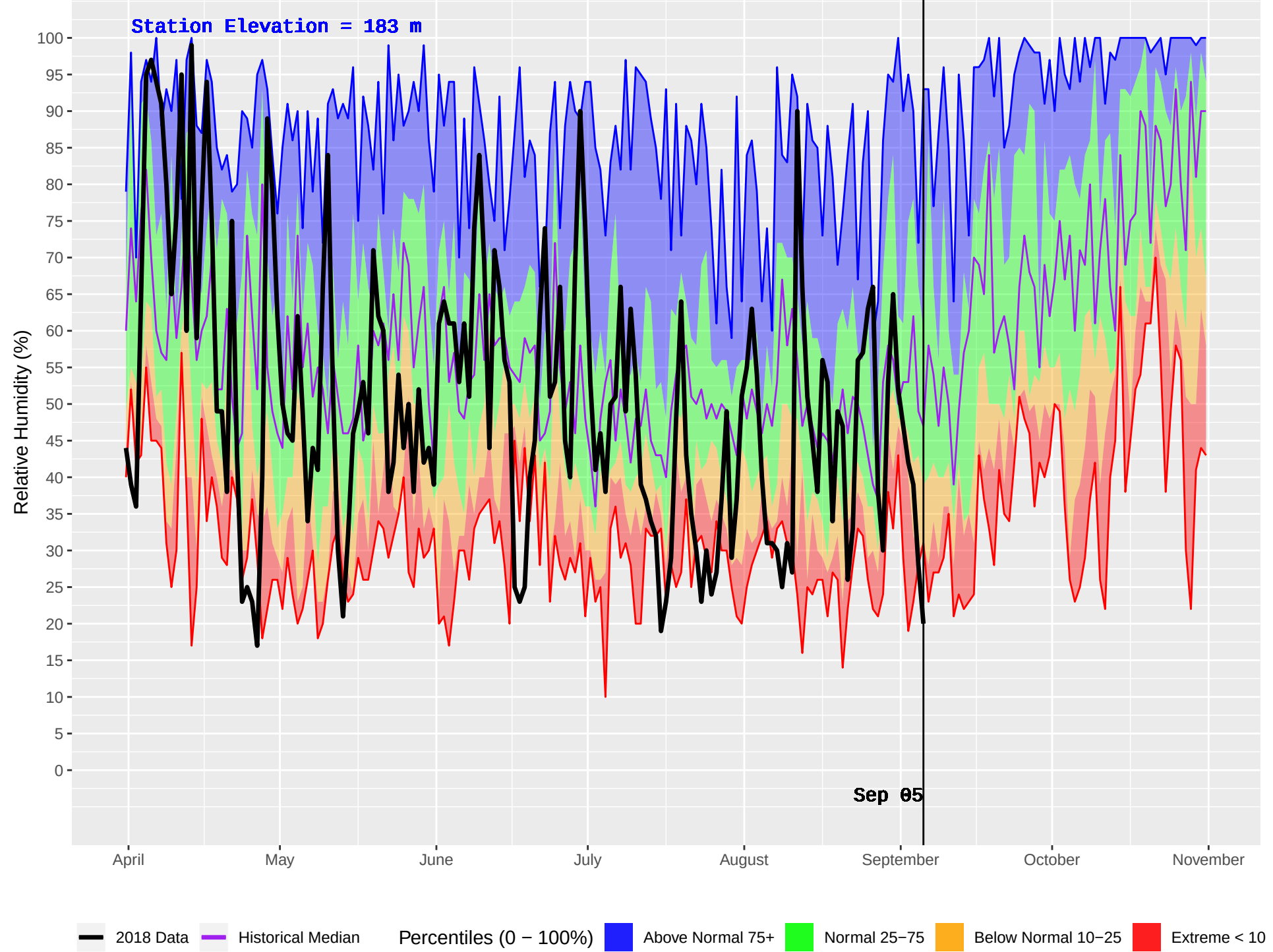
MESACHIE 2 (934) : Historical (2006–2016) and Current (2018) Daily Relative Humidity
