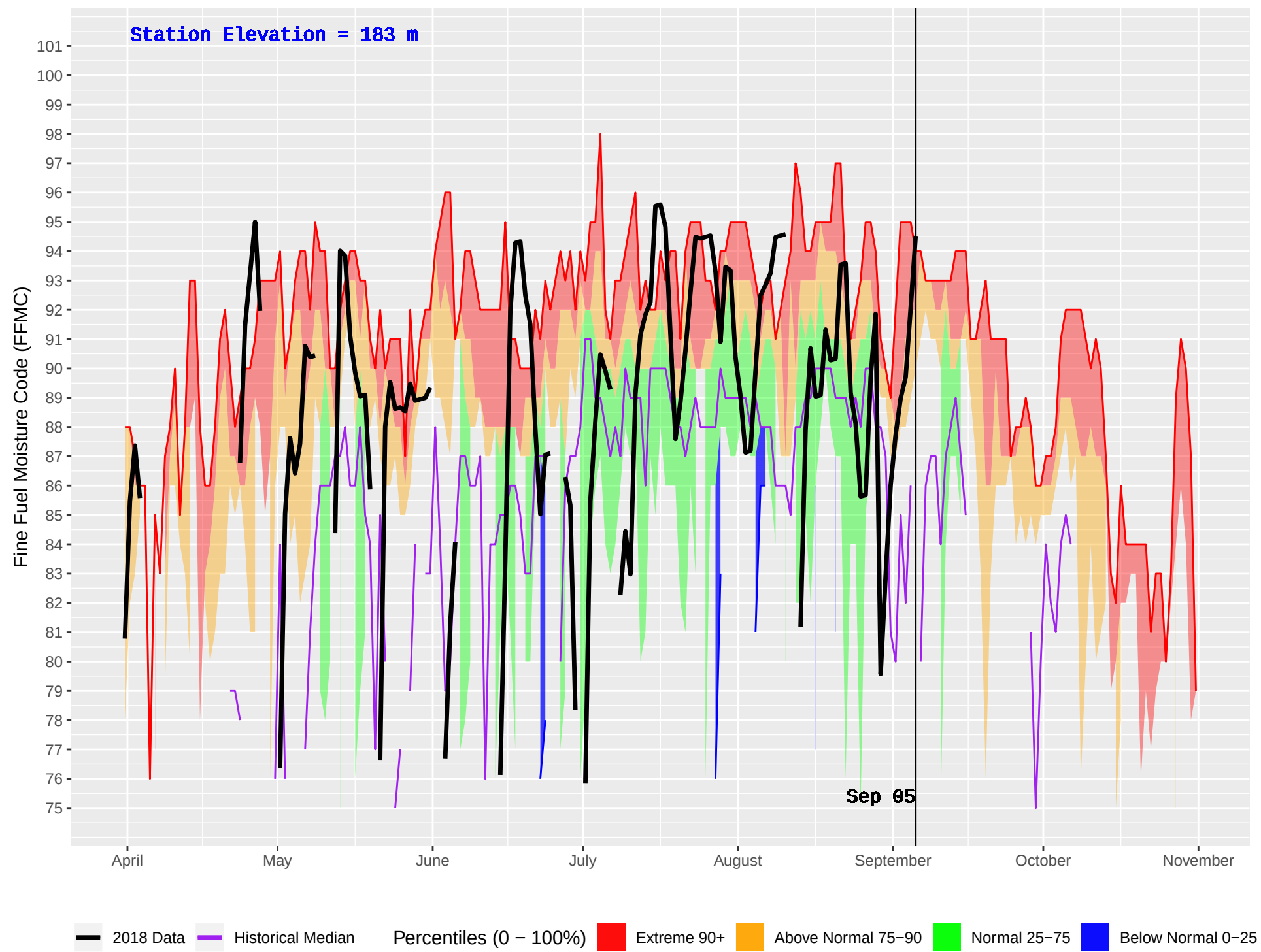
MESACHIE 2 (934) : Historical (2006–2016) and Current (2018) Daily Fine Fuel Moisture Code (FFMC)
